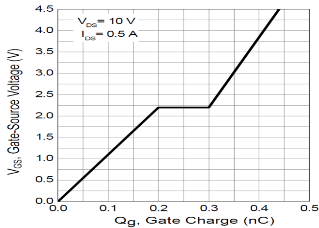
Fig. 9 Gate Charge
