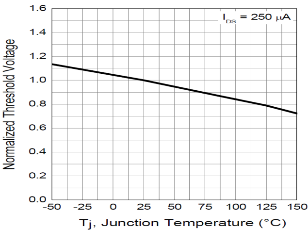
Fig. 8 Gate Threshold Variation vs. T j
