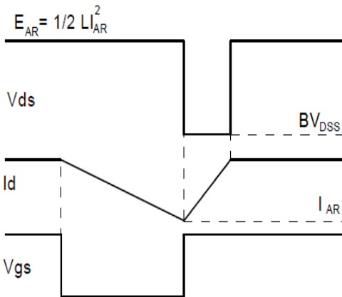
Fig.3-2 Avalanche waveform
